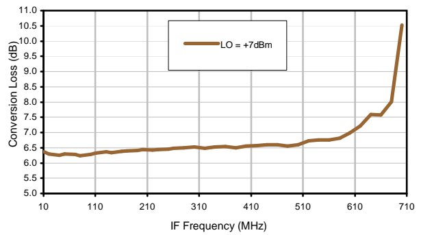
Conversion Loss vs. IF @ RF=805.5MHz
