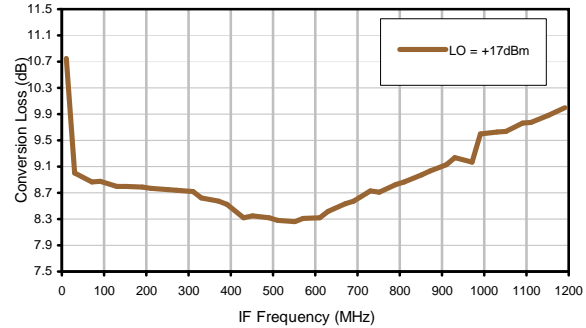
Conversion Loss vs. IF @ RF=1971MHz
