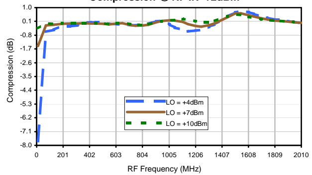
Compression @ RF IN=+2dBm
