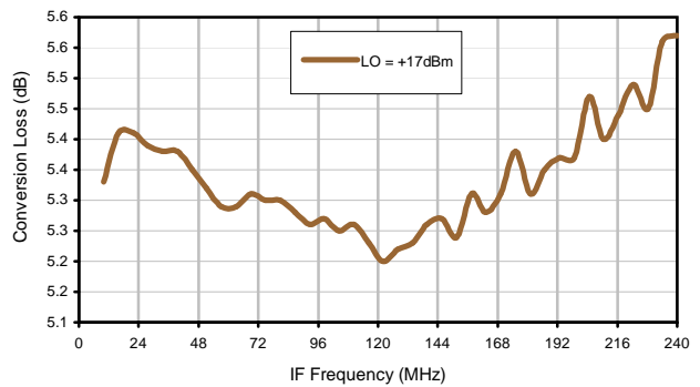
Conversion Loss vs. IF @ RF=250.1MHz
