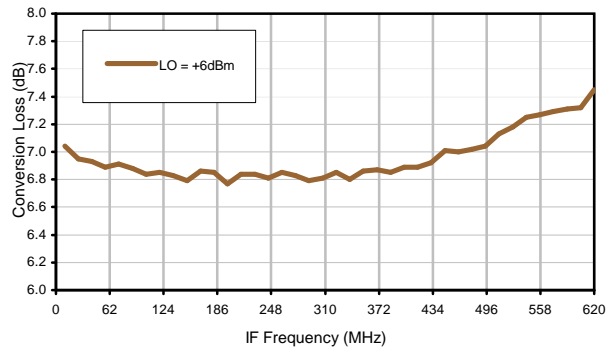
Conversion Loss vs. IF @ RF=630.1MHz
