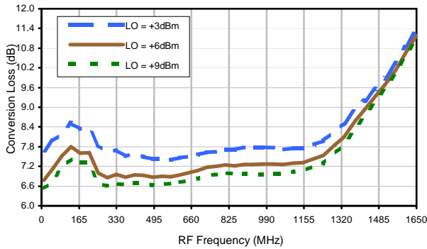
Conversion Loss @ IF=44.85MHz
