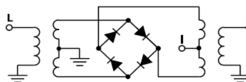
Electrical Schematic
