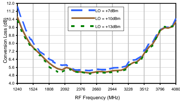
Conversion Loss vs. LO @ RF=2350MHz
