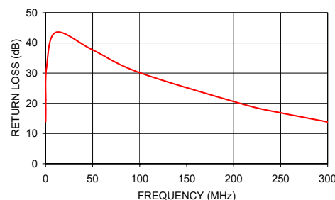
ADT4-6T INPUT RETURN LOSS
