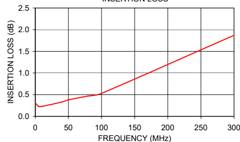
ADTT1.5-1 INSERTION LOSS
