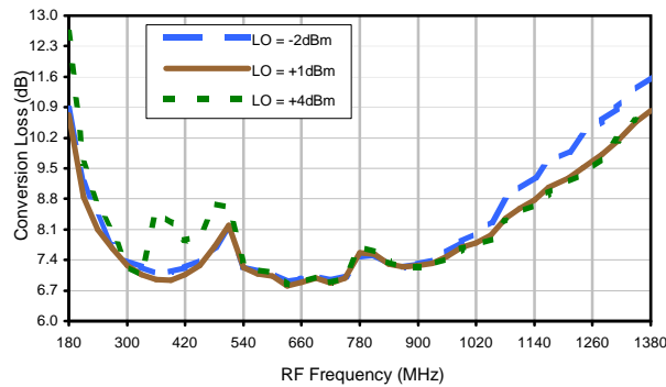
Conversion Loss vs. LO @ RF=832.5MHz
