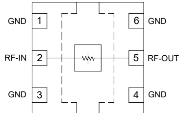
Figure 1. BAT-15+ Functional Diagram
