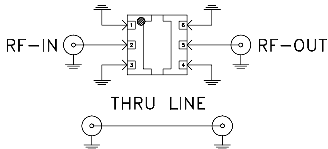
Schematic Diagram (Scale 5:1)
