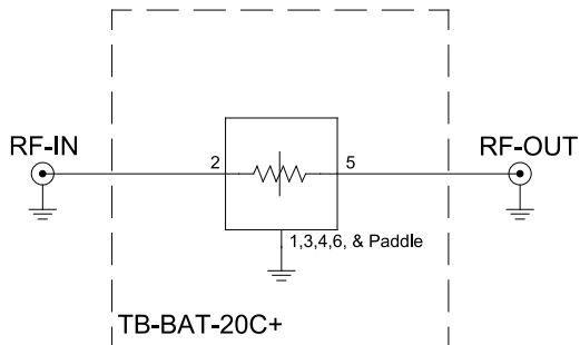
Figure 2. BAT-20+ Characterization and Application Circuit.
