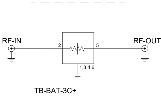
Figure 2. BAT-3+ Characterization and Application Circuit.
