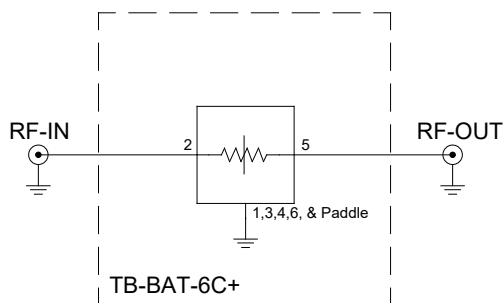
Figure 2. BAT-6+ Characterization and Application Circuit.
