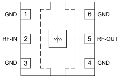
Figure 1. BAT-9+ Functional Diagram
