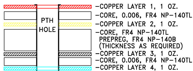
Stack-up Diagram
