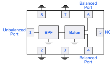
Figure 1. BBFCG2-252+ Functional Diagram
