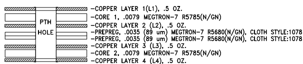
Figure 2. Suggested PCB Layout for BFHKI-5001+
