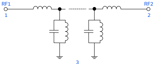
Figure 1. BFHKI-5001+ Functional Diagram
