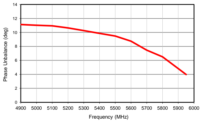
Phase Unbalance
