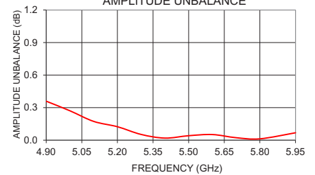
BLJC4-542R+ AMPLITUDE UNBALANCE
