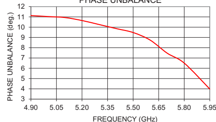
BLJC4-542R+ PHASE UNBALANCE
