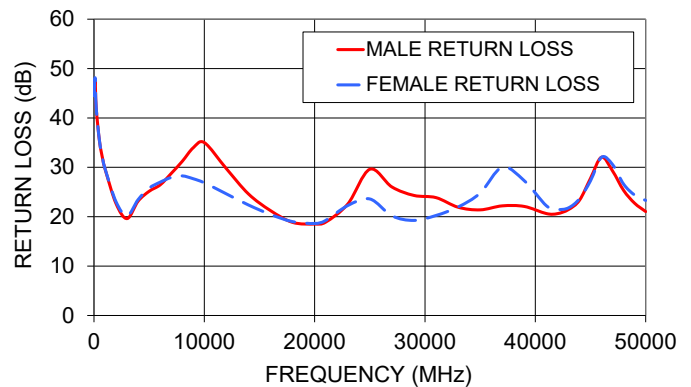
BLK-V54+ RETURN LOSS
