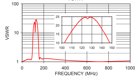
BSF-C125+ VSWR
