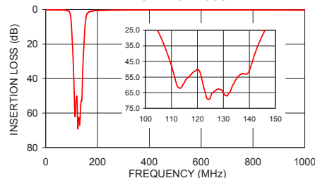
BSF-C125+ INSERTION LOSS
