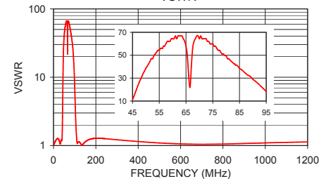
BSF-C70+ VSWR
