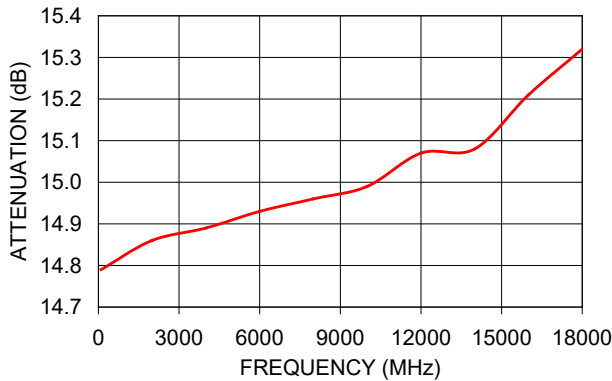
BW-N15W5+ ATTENUATION
