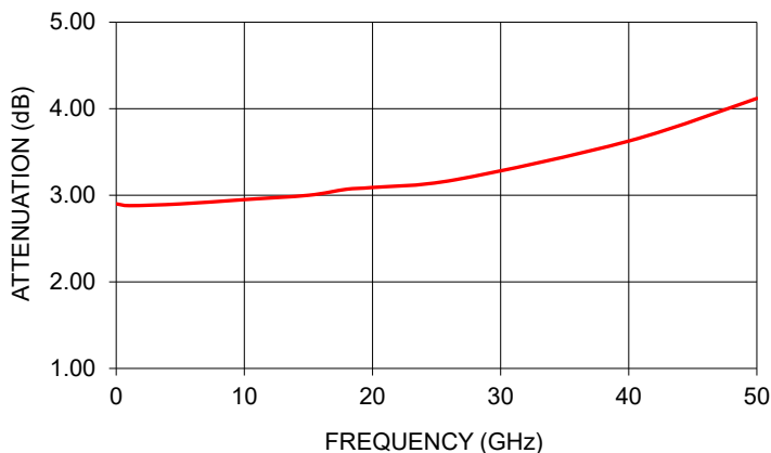
BW-V3-1W54+ ATTENUATION
