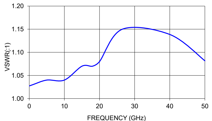
BW-V3-1W54+ VSWR
