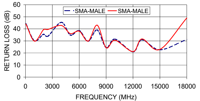
CBL-1.5FT-SMSM+ RETURN LOSS
