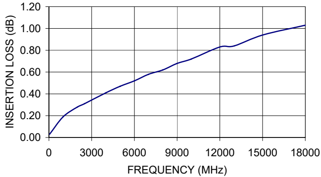
CBL-1.5FT-SMSM+ INSERTION LOSS
