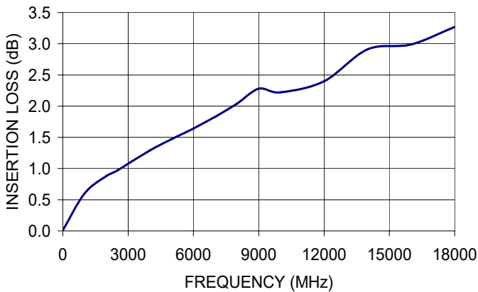
CBL-1.5M-NMNM+ INSERTION LOSS
