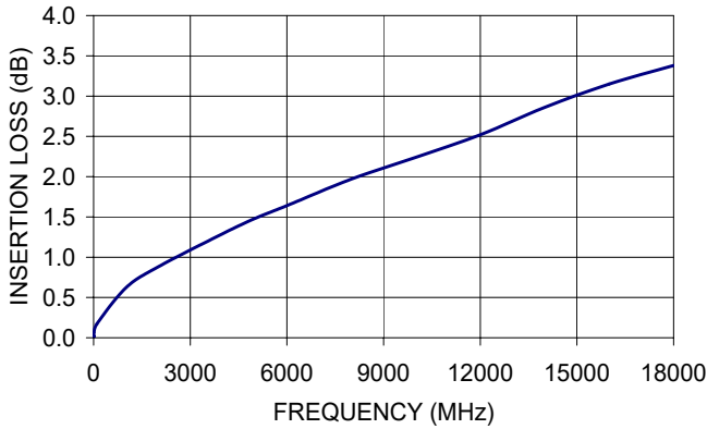
CBL-5FT-NMNM+ INSERTION LOSS
