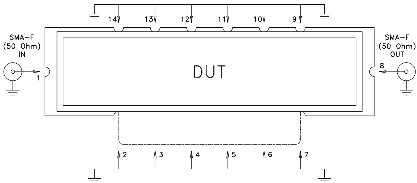
Schematic Diagram
