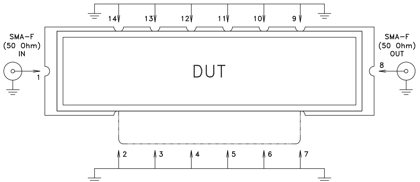
Schematic Diagram
