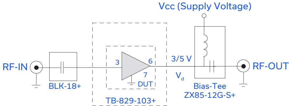
Fig 1. Block Diagram of Test Circuit used for characterization. (DUT tested on Mini-Circuits Characterization test board TB-829-103+) Gain, Return Loss, Output Power at 1 dB Compression (P1dB), Output IP3 (OIP3) and Noise Figure measured using Agilent's N5242A PNA-X microwave network analyzer.
