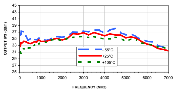
OUTPUT IP3 vs. FREQUENCY & TEMPERATURE OUTPUT POWER = 0 dBm/1tone, Vd = 3V
