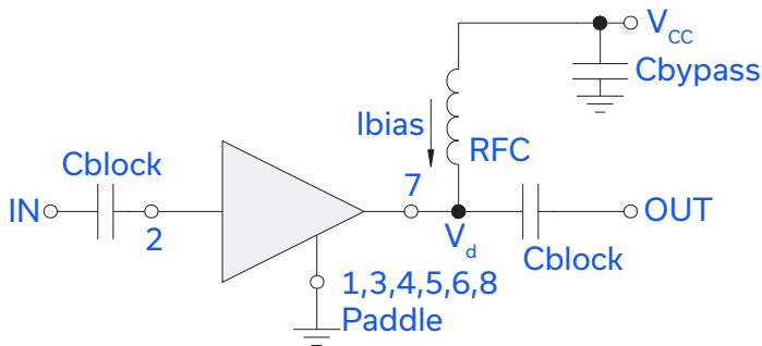
Fig 1. Block Diagram of Test Circuit used for characterization. (DUT soldered on Mini-Circuits Test Board TB-829-81+) Gain, Output Power at 1 dB Compression (P1dB) and Output IP3 (OIP3) are measured using R&S Network Analyzer ZVA-24. Noise Figure measured using Agilent's N5242A PNA-X microwave network analyzer.
