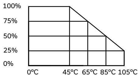
Power Derating 4 vs Temperature
