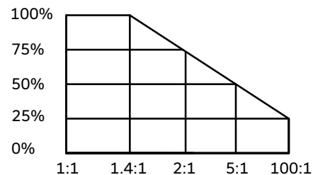
Power Derating 4 vs VSWR
