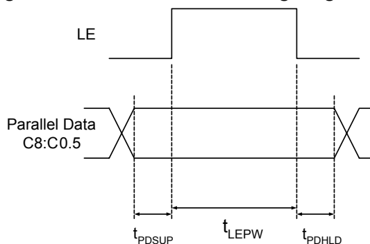
Figure 1: Parallel Interface Timing Diagram
