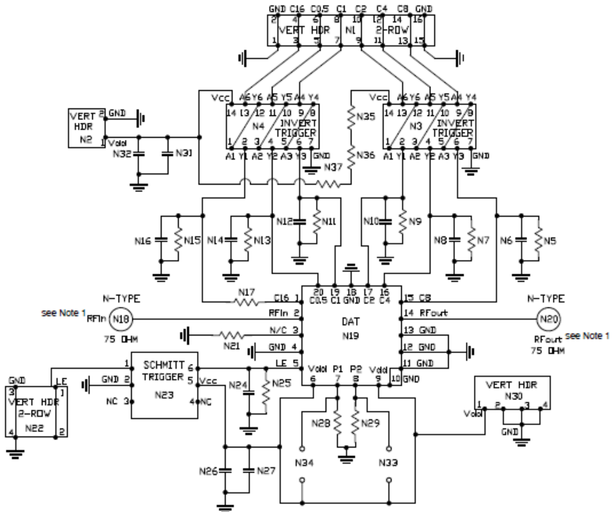
TB-337 Evaluation Board Schematic Diagram
