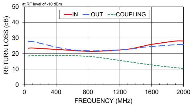
RETURN LOSS
