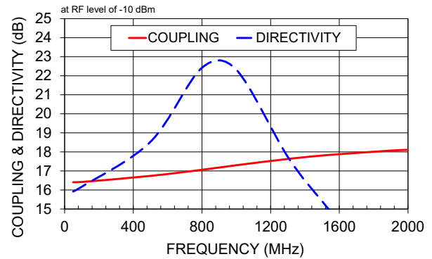
COUPLING & DIRECTIVITY
