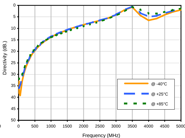
Directivity vs. TEMPERATURE
