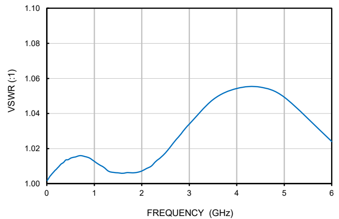
N MALE VSWR (+25 °C)
