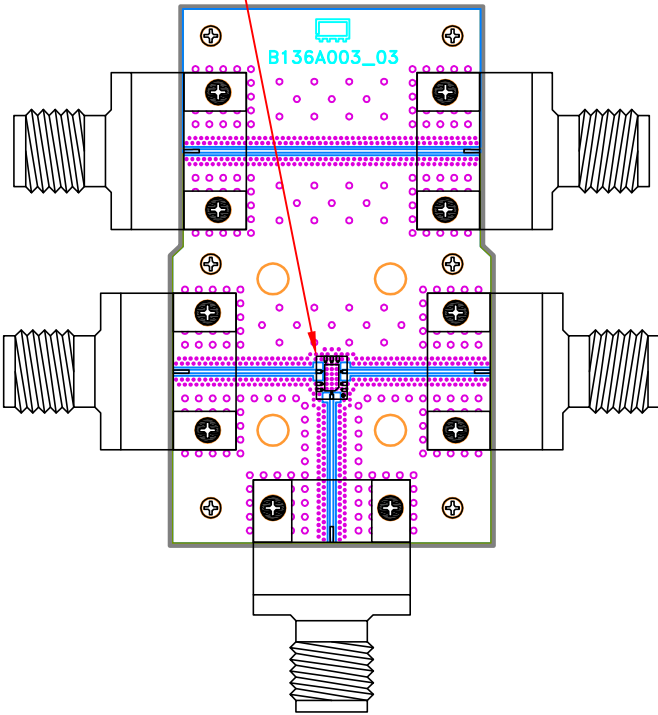
DETAIL "A" LOCATION OF INTERCONNECTOR AND UNITS COMPONENTS (SCALE 5:1)
