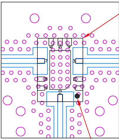
DETAIL "A" LOCATION OF INTERCONNECTOR AND UNITS COMPONENTS (SCALE 5:1)
