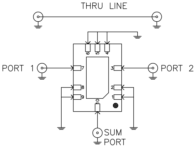
SCHEMATIC DIAGRAM
