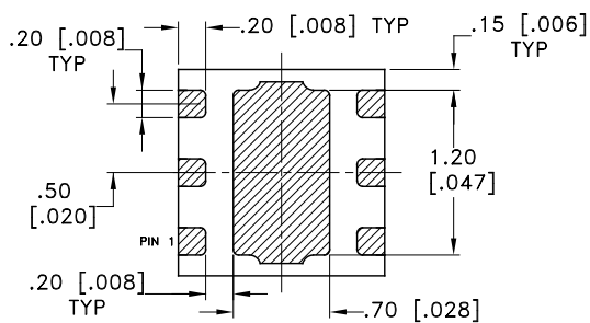
BOTTOM VIEW
