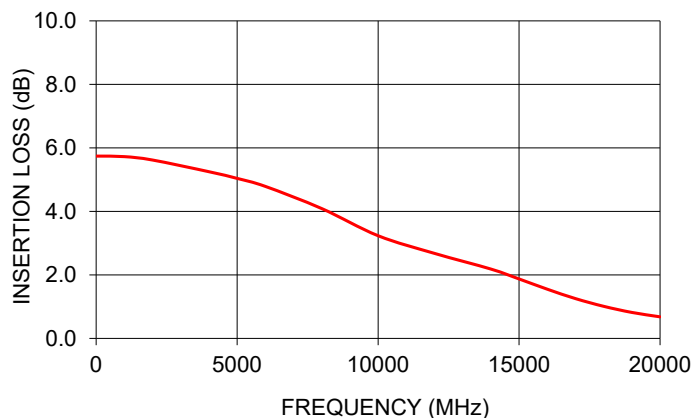
EQY-5-24+ INSERTION LOSS
