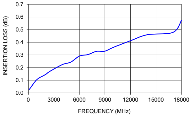
FL086-6SM+ INSERTION LOSS
