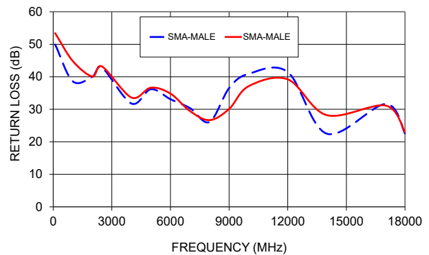
FL086-6SM+ RETURN LOSS
