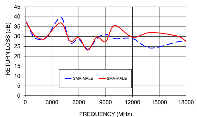
FL141-6SM+ RETURN LOSS
