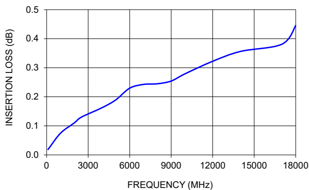
FL141-6SM+ INSERTION LOSS
