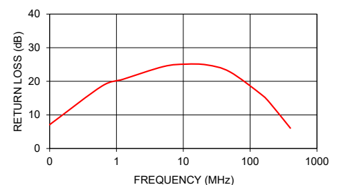
FT-1.5-1+ INPUT RETURN LOSS
