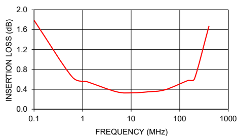
FT-1.5-1+ INSERTION LOSS
