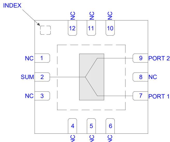
Figure 1. GP2XA+ Functional Diagram
