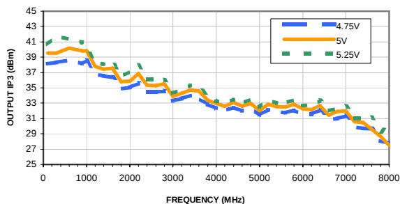
OUTPUT IP3 vs. FREQUENCY & DEVICE VOLTAGE OUTPUT POWER = 0 dBm/100W, Temperature = +25°C
