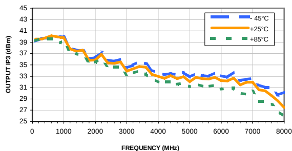
OUTPUT IP3 vs. FREQUENCY & TEMPERATURE OUTPUT POWER = 0 dBm/100µV, Vd = 5.00V
