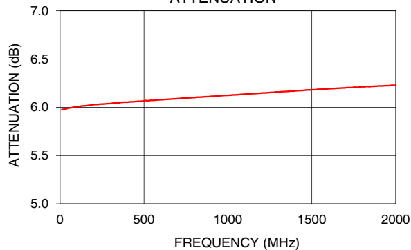
HAT-6A+ ATTENUATION
