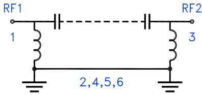
Figure 1. HFCG-740+ Functional Diagram
